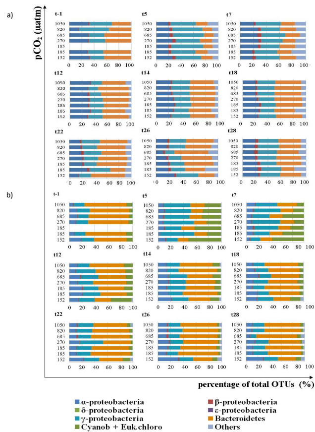
Fig. 2. Microbial community overview of the most abundant phyla in (a) the small (0.2–3 μm) and (b) the large (3–12 μm) size fraction during t-1 , t5 , t7 , t12 , t14 , t18 , t22 , t26 and t28 ; x-axis represents percentage of total OTUs and y-axis represents p\text{CO}_2 in \mu\text{atm}
