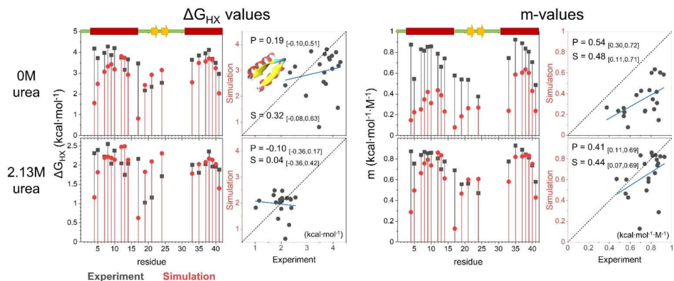
Figure 7. Comparison of the experimental and simulated \Delta G_{HX} and m -values for HEEH_rd4_0097.
