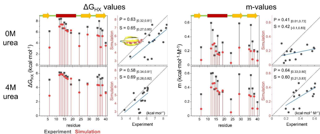
Figure 6. Comparison of the experimental and simulated \Delta G_{HX} and m -values for EHEE_rd2_0005. Values from experiment and simulation are compared in the absence and presence of denaturant. The corresponding secondary structure is shown on the upper left (strands in yellow, helices in red). The correlation is shown on the right in each panel. The blue line is the best fit line. The Pearson ( P ) and Spearman ( S ) correlation coefficients and the 90% confidence interval (in the parentheses) are provided.
